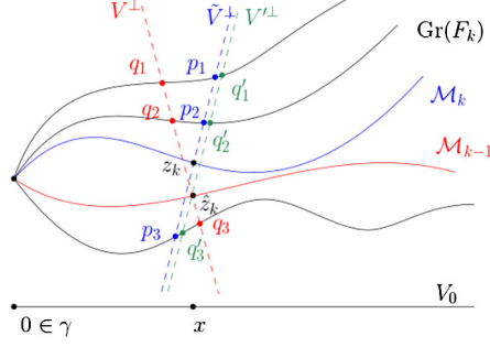
FIG. 4. — An illustration of how Lemma 17.3 is used
