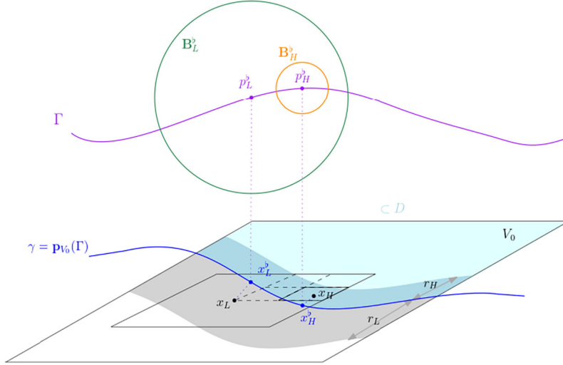
FIG. 3. — An illustration of the various relevant points in the Whitney square
