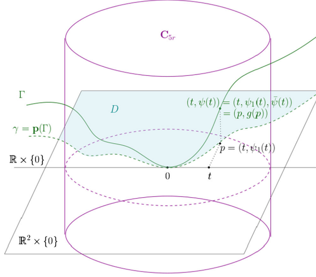
FIG. 2. — An illustration of the maps describing the boundary
