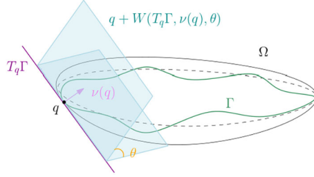
FIG. 1. — An illustration of the wedge where V is the tangent T_q \Gamma to \Gamma at some boundary point q , whereas \nu the interior unit normal \nu(q) to the convex barrier \Omega at q
